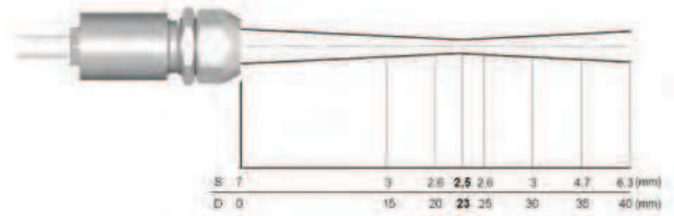
2:1 optics with CF-lens
