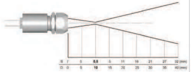
15:1 optics with CF-lens
