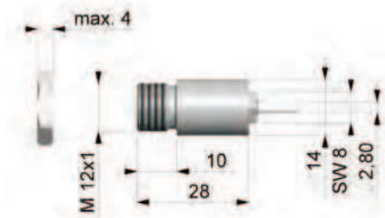
Dimensions CSmicro
